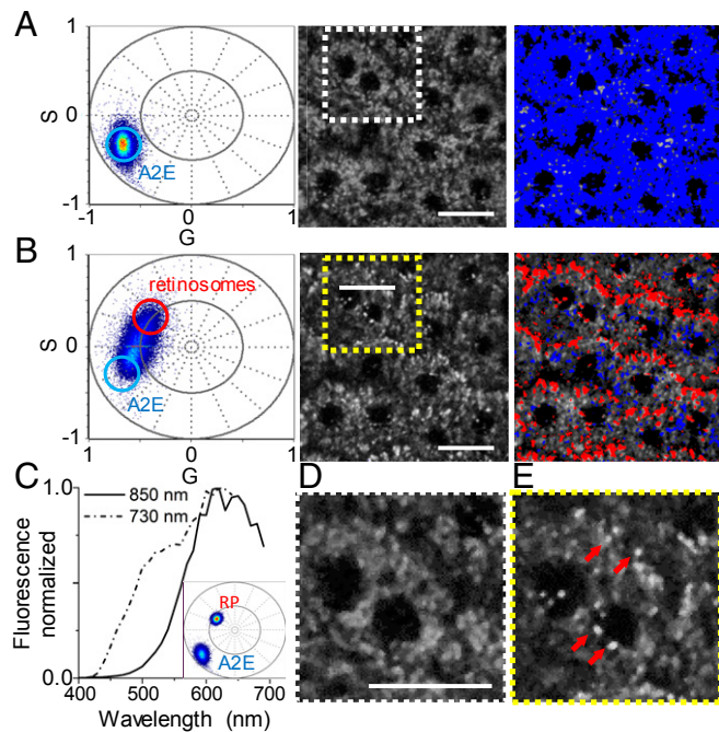
Fig. 3. Spectral analysis distinguishes retinosomes and A2E within RPE cells in albino Abca4 FPV/FPV Rdh8 -/- mouse eye without staining. (A) Data obtained with 850-nm excitation wavelength. (B) Data obtained with 730-nm excitation. (A and B, Left ) Spectral phasor plots. (A and B, Center ) TPE fluorescence intensity-based images. (A and B, Right ) Pseudocolor images obtained by applying the cursor selection in the spectral phasor plots shown in A and B, Left . Dashed-lined squares outline regions presented in higher zoom-in in D and E. (C) Normalized fluorescence emission spectra for 850- and 730-nm excitation from the RPE. ( Inset ) Spectral phasor of pure retinal palmitate and 10 mM A2E in DMSO. RP, retinyl palmitate. (D) Zoomed-in image of RPE with 850-nm excitation. (E) Zoomed-in image of RPE with 730-nm excitation. Red arrows point to exemplary particles which light up with 730-nm excitation. (Scale bars, 20 \mu m.)
